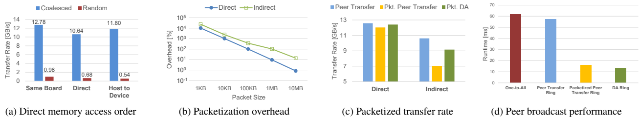
Figure 2: Inter-GPU Memory Transfer Microbenchmarks
