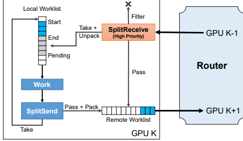
Figure 9: Distributed Worklist Implementation
