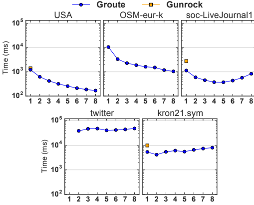
Figure 11: PageRank Execution Time
