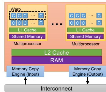
Figure 4: Single GPU Architecture
