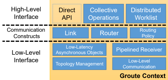
Figure 7: The Groute Library
